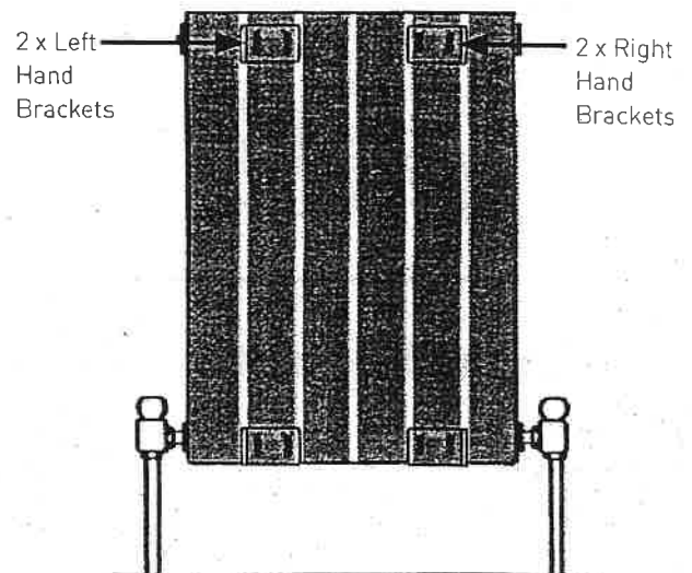
Drawing 2 - Bracket Positions
